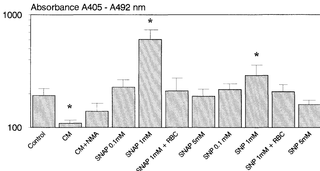
Fig. 2. BrdU incorporation assay of WI38 cells cultured for 24 h under various conditions. After cytokine stimulation (CM) proliferation was significantly reduced, whereas addition of 1 mM S -nitroso- N -acetylpenicillamine (SNAP) or 1 mM nitroprusside (SNP) led to an increased proliferation (* P < 0.001 as compared to control). RBC: red blood cells.
